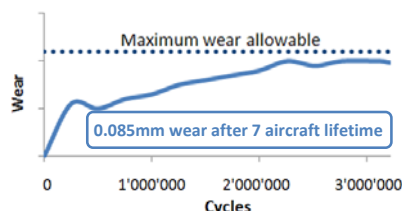
Duty cycles \pm 5^\circ , 120MPa, ball \phi 77.9mm
